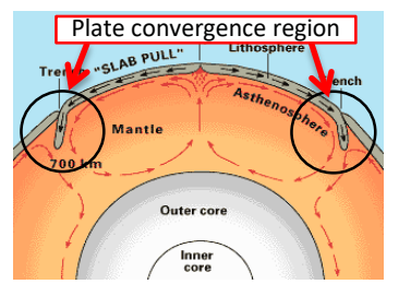
Mantle convection
